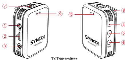
TX Transmitter
